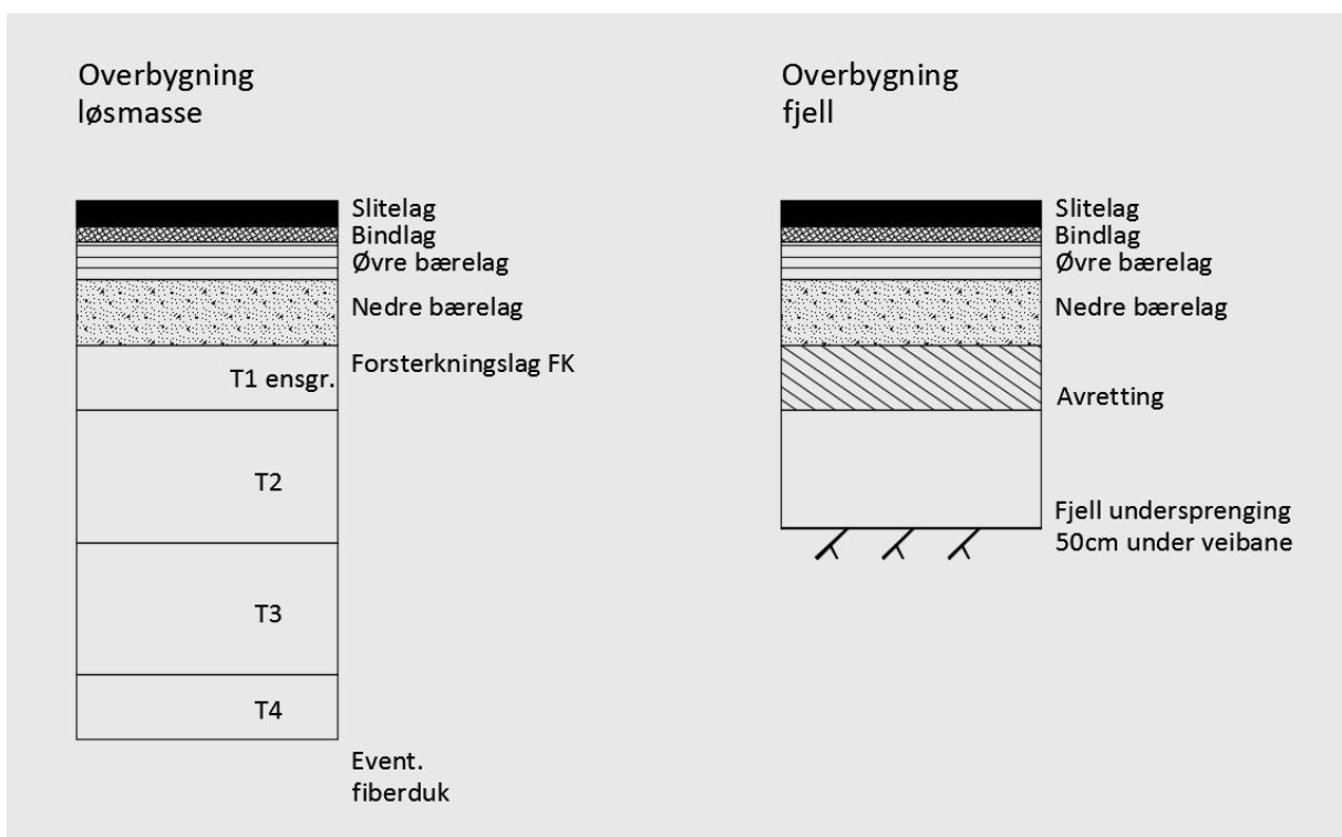
Figur 17 overbygning
